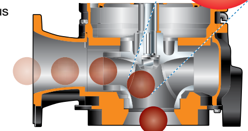
Shrouded Channel Impeller
