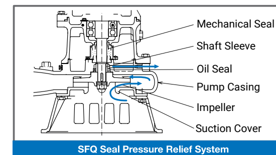
SFQ Seal Pressure Relief System
